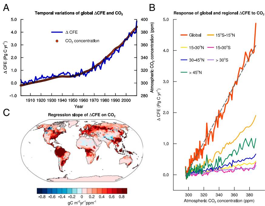
Fig. 1. Temporal and spatial variations of the difference in the \text{CO}_2 fertilization effect ( \Delta\text{CFE} , \text{PgC/y} ) on annual gross primary production simulated with CLM4.5 between including and lacking explicit consideration of mesophyll conductance ( g_m ). (A) Historical trends in \Delta\text{CFE} (blue curve, left ordinate) and in atmospheric \text{CO}_2 concentration (ppm, red dots, right ordinate) from 1901 to 2010. (B) The variation of the global and latitudinal \Delta\text{CFE} with atmospheric \text{CO}_2 concentration. The global curve (red) is fitted with a line ( y = -13.55 + 0.05x , r^2 = 0.98 ). (C) The spatial variation in the slope ( \text{gC/m}^2/\text{y/ppm} ) of the linear regression of the grid-based \Delta\text{CFE} as a function of atmospheric \text{CO}_2 concentration. The increase of \Delta\text{CFE} with time and atmospheric \text{CO}_2 concentration demonstrates that carbon cycle models without explicit representation of mesophyll diffusion underestimate \text{CO}_2 fertilization effect.
