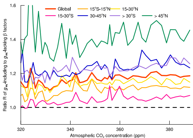
Fig. 2. Changes with atmospheric \text{CO}_2 concentration of the global and latitudinal ratio ( R ) of the \beta factors calculated with CLM4.5 between including and lacking explicit consideration of mesophyll conductance ( g_m ). R fluctuates erratically for the first half of the 20th century when the atmospheric \text{CO}_2 is close to the baseline reference of 296 ppm in 1901, causing the denominator of R to vary around zero. Therefore, values of R when the atmospheric \text{CO}_2 is less than 320 ppm are not shown. The dashed line at R = 1 separates the underestimation ( R > 1 ) from the overestimation ( R < 1 ) of the \text{CO}_2 fertilization effect on gross primary production by CLM4.5 lacking g_m compared with CLM4.5 including g_m .
